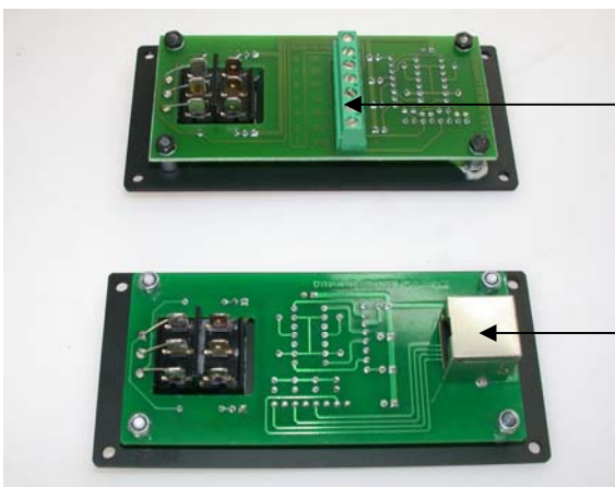
P30114 Panel with cable clamp
